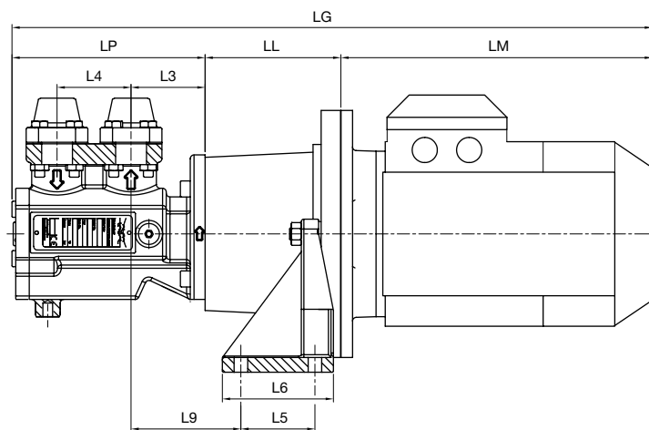
Pump type ALP 0015–0085
